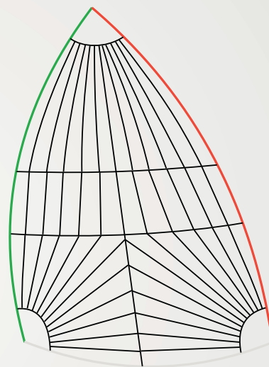
Coloured braids to differentiate port to starboard when the spinnaker is in its bag
